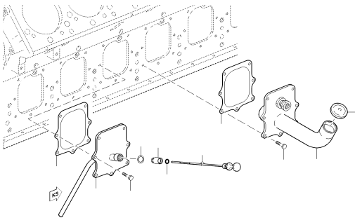
INSPECT PORT COVER FOR OIL DIPSTICK 010.00390
